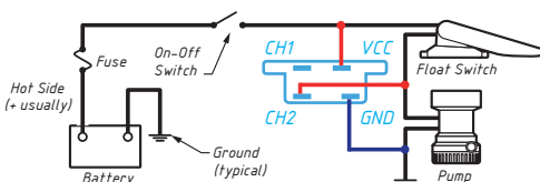
Pic. 1. Wiring diagram from the Rule Industries
